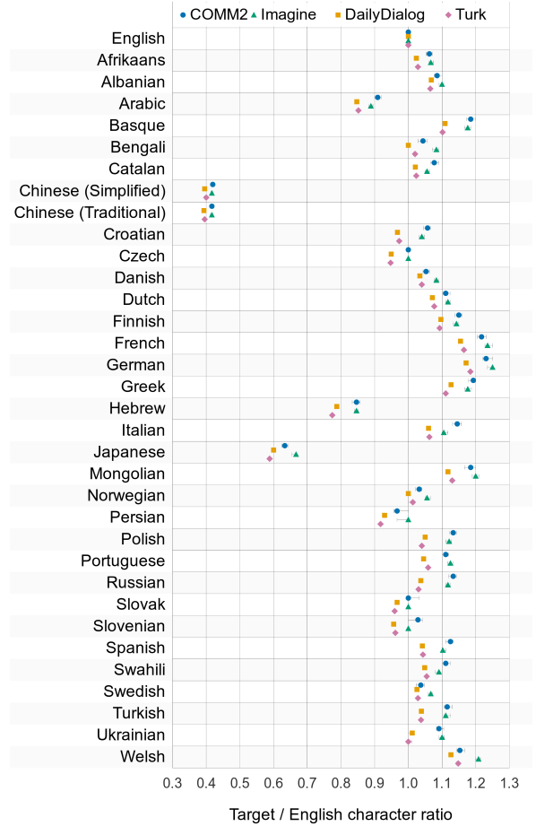
Figure 1: Median target-to-English non-whitespace character ratios by language and dataset. Error bars show 95% bootstrap confidence intervals.
