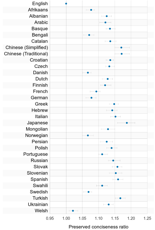
Figure 2: Preservation of COMM2 conciseness after translation. Points are the median preserved-conciseness ratio. Error bars show 95% bootstrap confidence intervals. A ratio of 1 means the proportional reduction from full to concise was preserved exactly; values above 1 indicate some conciseness was lost.
